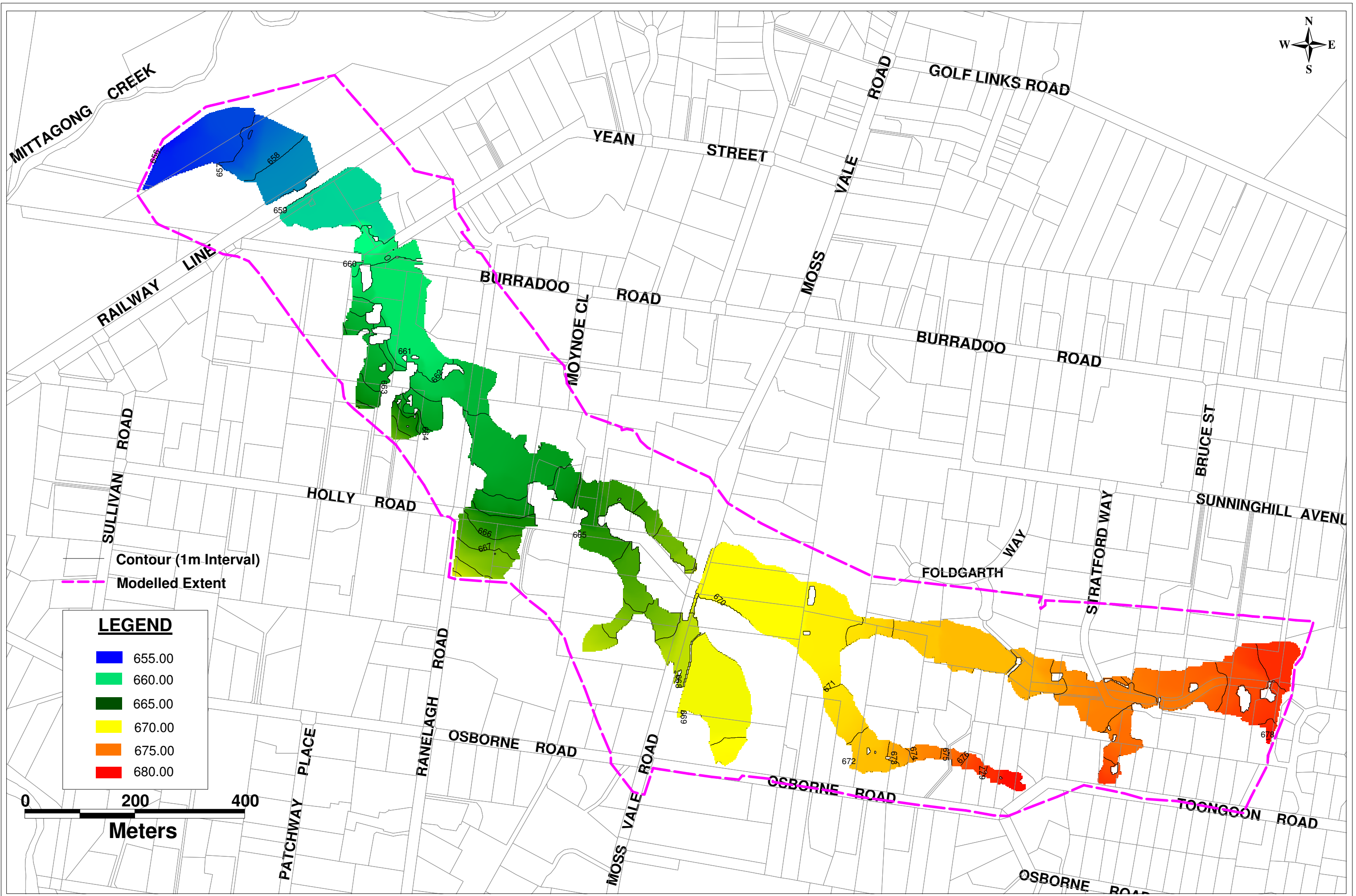
FIGURE 7.3 50YearARI_PeakWaterLevel
