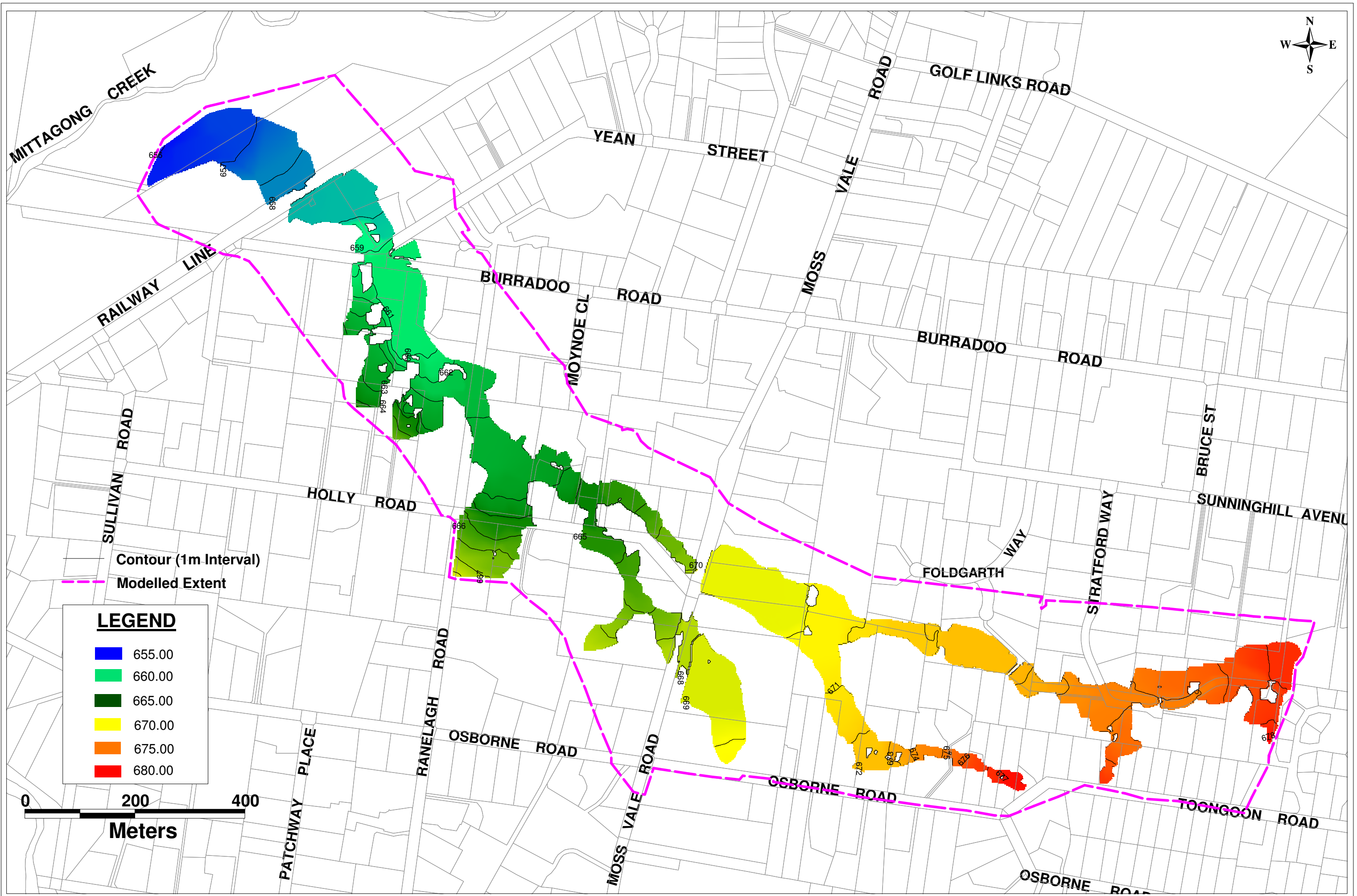
FIGURE 7.5 5YearARI_PeakWaterLevel
