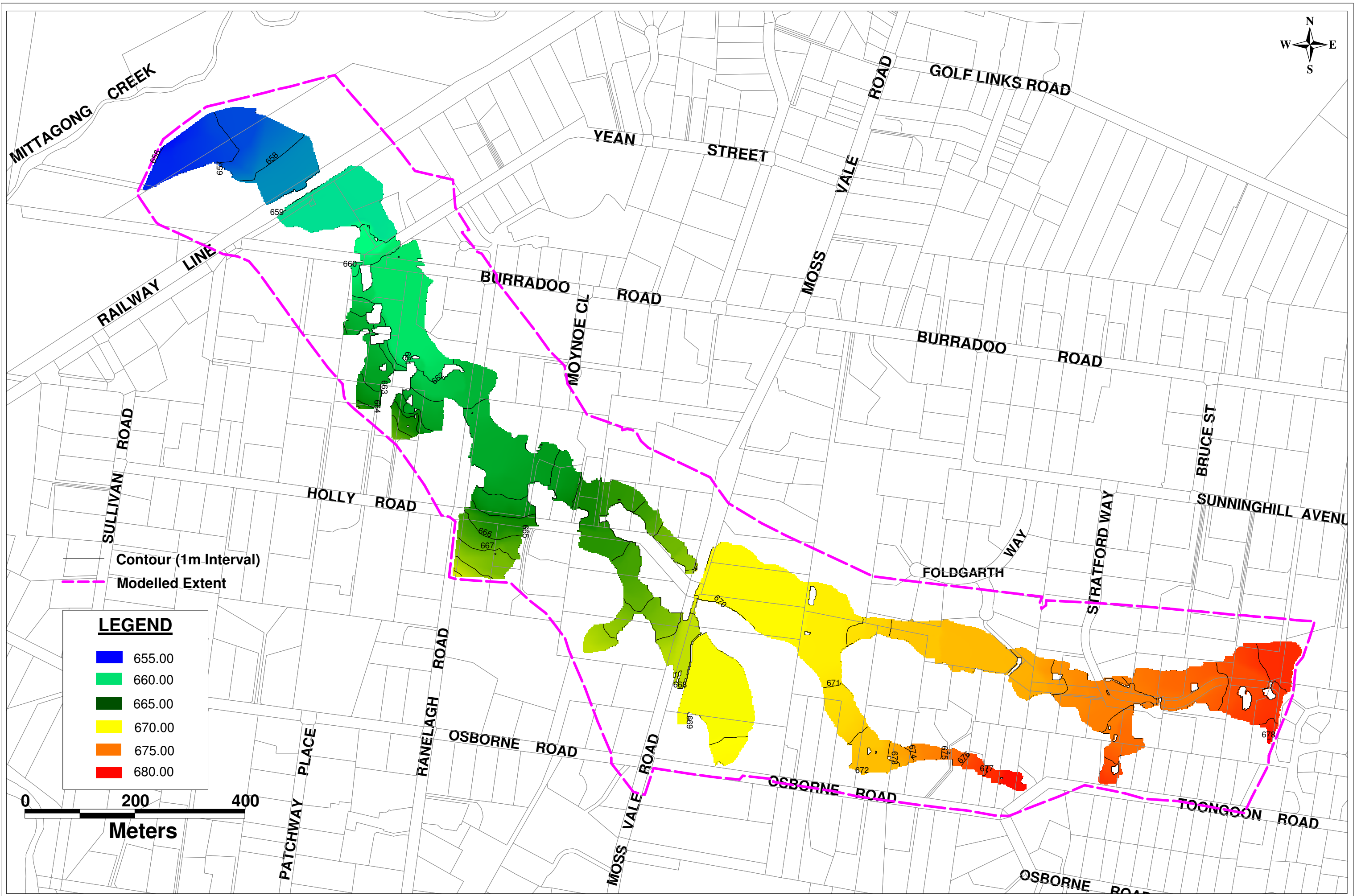
FIGURE 7.2 100YearARI_PeakWaterLevel
